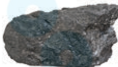
Figure 7.1 Natural magnet
