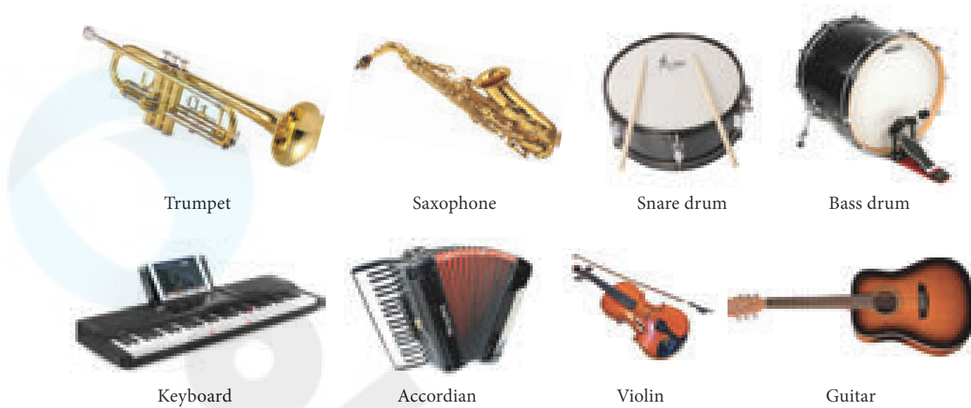
Figure 6.4 Musical instruments
