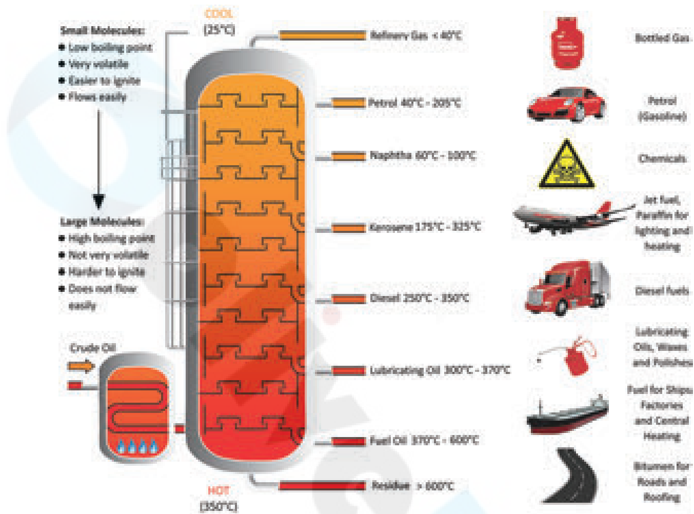
Figure 15.17 Product obtained from petroleum
