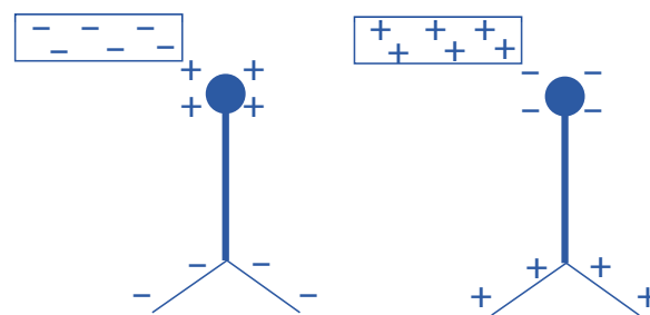
Figure 5.7 Movement of charges in electroscope near the top knob of the electroscope, the free electrons in the electroscope start to move up towards the knob. This means that the bottom has a net positive charge. The leaves will spread apart again now.
