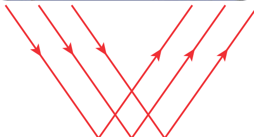
Figure 3.7 Regular reflection
