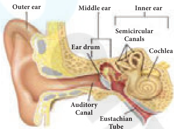
Figure 6.6 Human Ear
